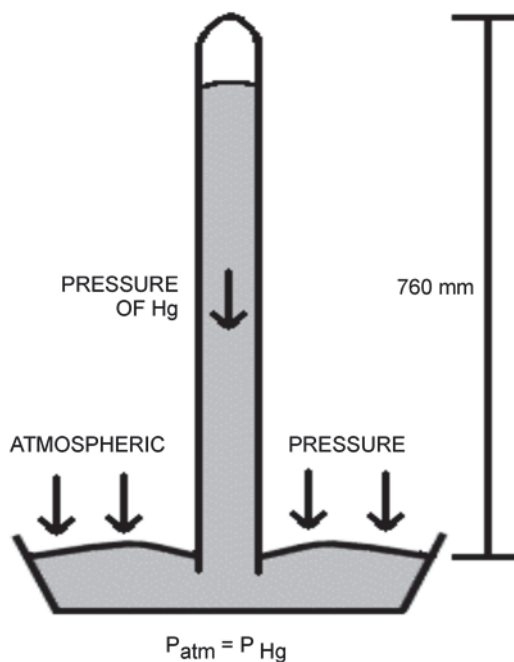
Figure 13-3-1 Barometer
